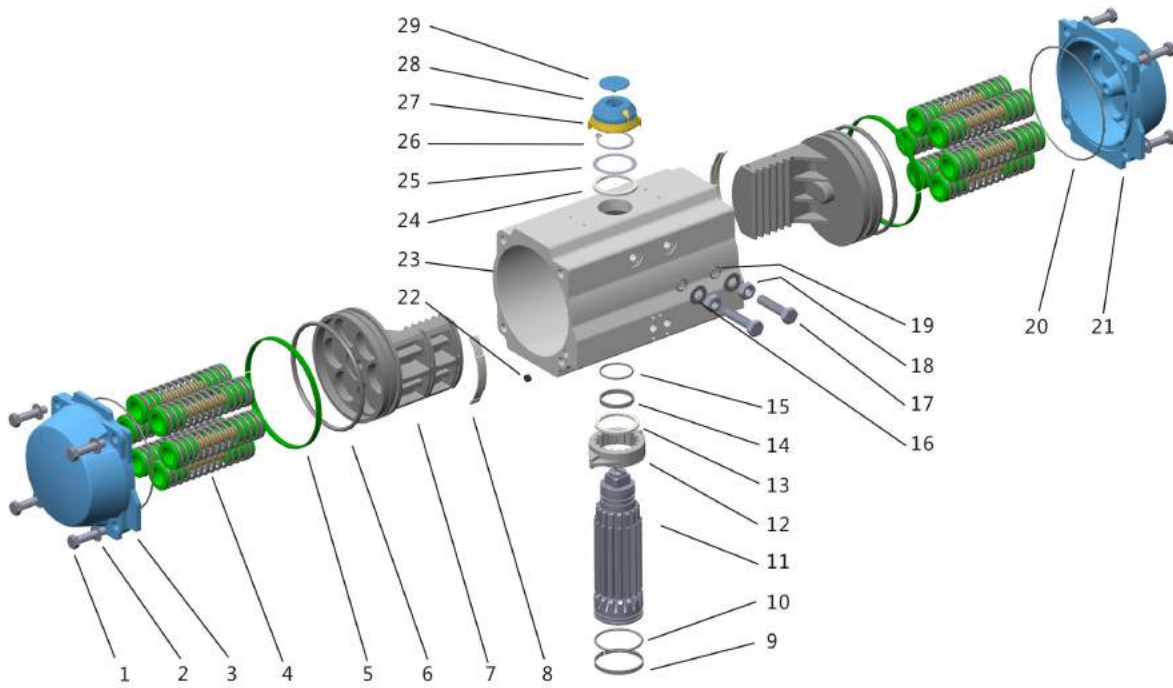
零部件明细表 Components Material
